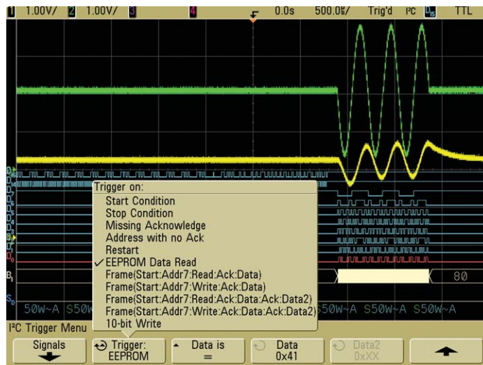
Figure 12. Triggering on a 3-cycle chirp with I 2 C triggering and decode in an Agilent MSO.
